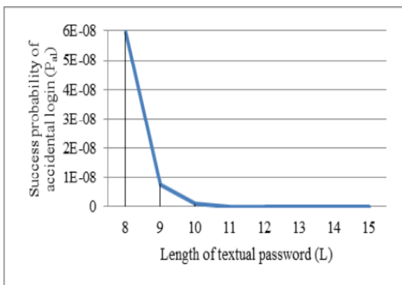
Fig. 4: The success probability of accidental login for different values of L .
