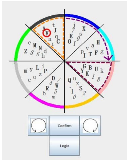
Fig. 3. The user has to rotate the sector (marked with orange dotted line for illustration only) containing K_i (marked with small red circle for illustration only) into his pass-color sector (marked with brown dotted line for illustration).
