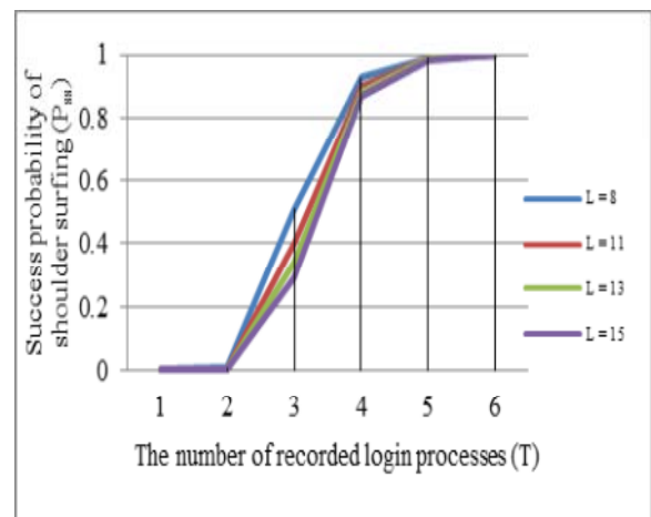
Fig. 5: The success probability of shoulder surfing for T times login process records and different values of L .
